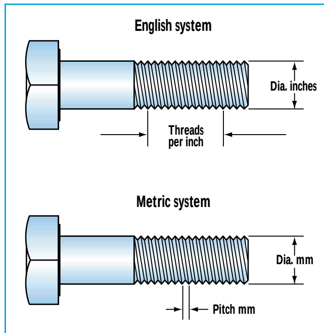
2. English and metric systems of measuring threads and bolt diameter
