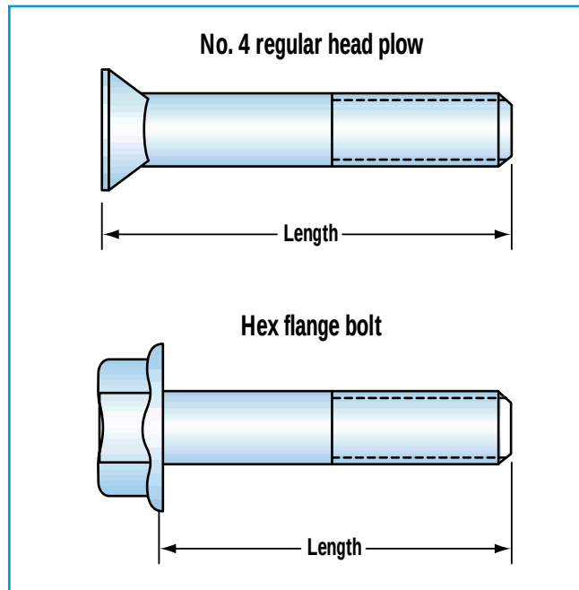
1. Two common refiner plate bolts—a regular head plow and a hex flange bolt—and the method of measuring bolt length for each
