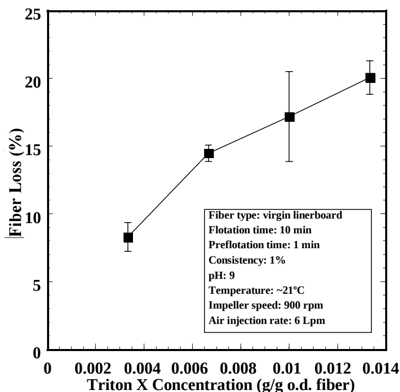
Figure 4. Effect of TX-100 concentration on fiber loss
