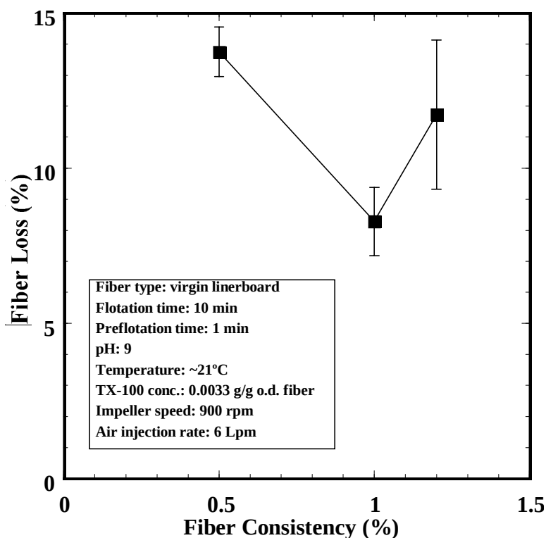
Figure 6. Effect of flotation consistency on fiber loss
