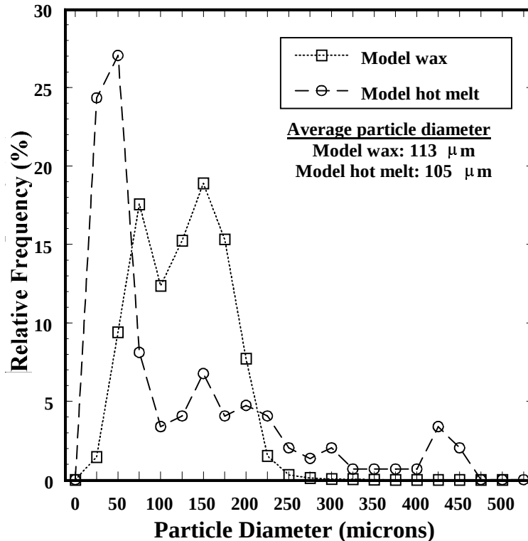
Figure 2. Initial particle size distributions of the model wax and hot melt
