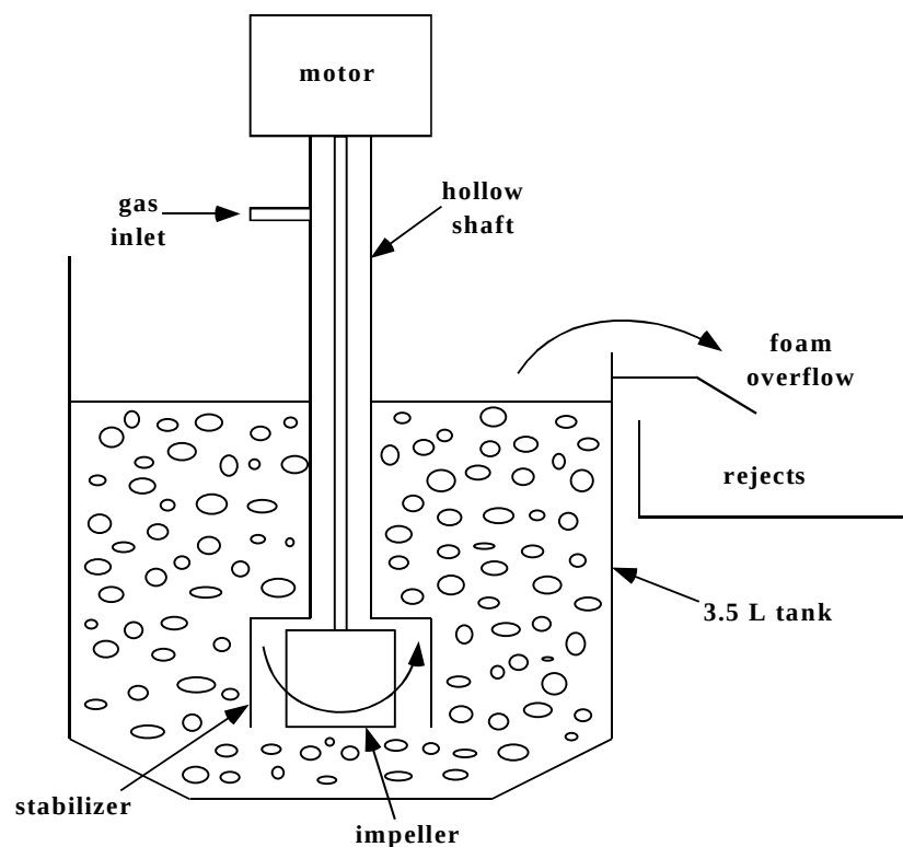
Figure 1. Wemco flotation cell
