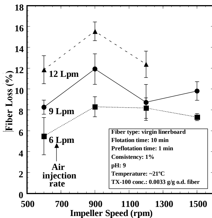
Figure 7. Effect of impeller speed and air injection rate on fiber loss
