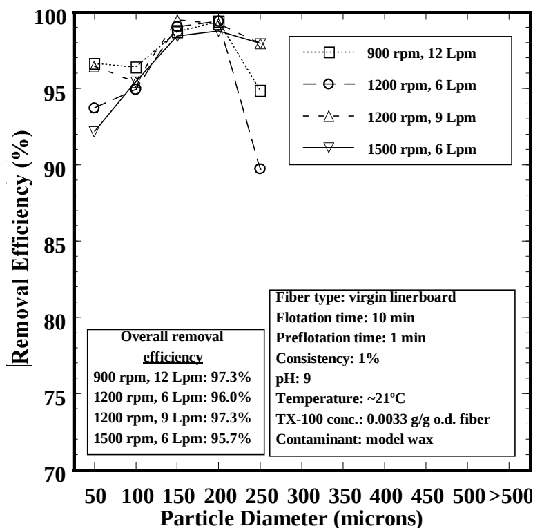
Figure 8. Model wax removal efficiency for various combinations of impeller speed and air injection rate
