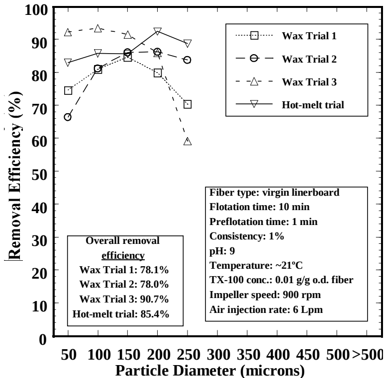
Figure 3. Model wax and hot-melt removal efficiencies for the flotation reference conditions
