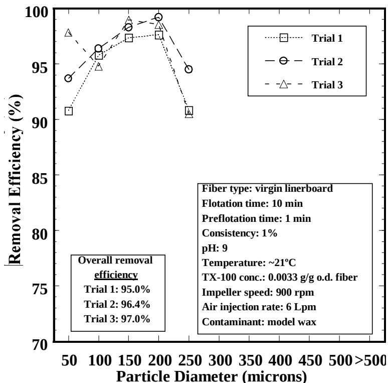
Figure 5. Model wax removal efficiency at a TX-100 concentration of 0.0033 g/g o.d. fiber
