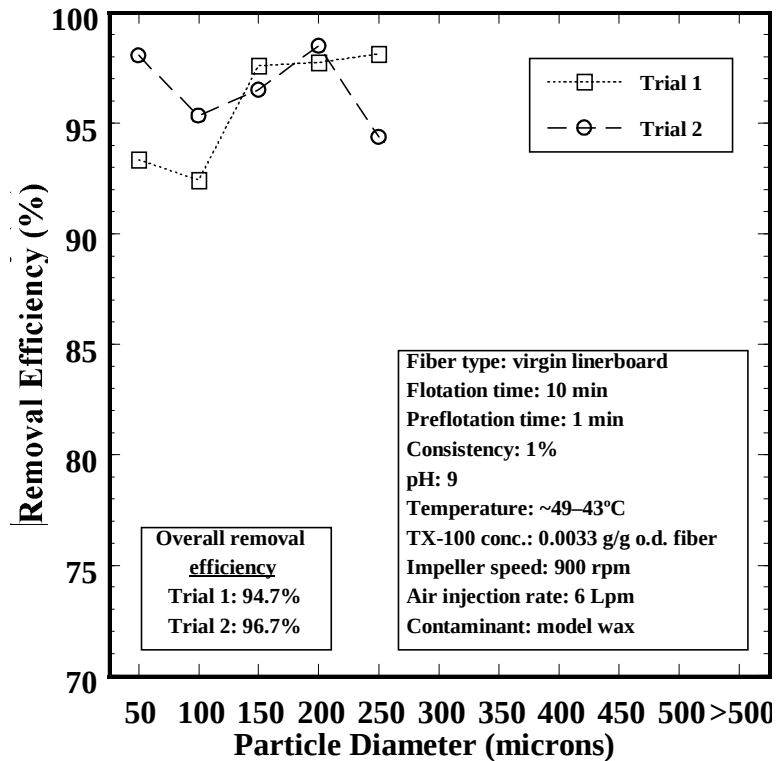
Figure 9. Model wax removal efficiency at an elevated flotation temperature
