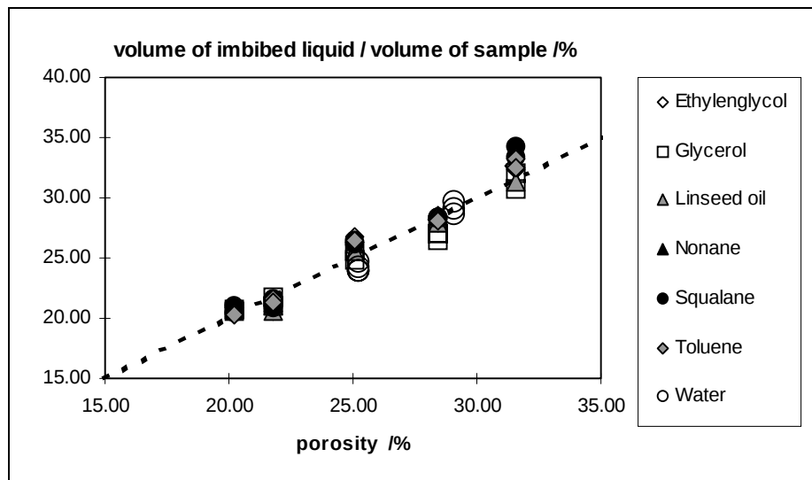
Fig. 8. One-to-one correlation of imbibed liquid volume with porosity for both the polar and apolar fluids as determined from the generalized correspondence shown in Fig. 7, including water at two arbitrarily chosen porosities
