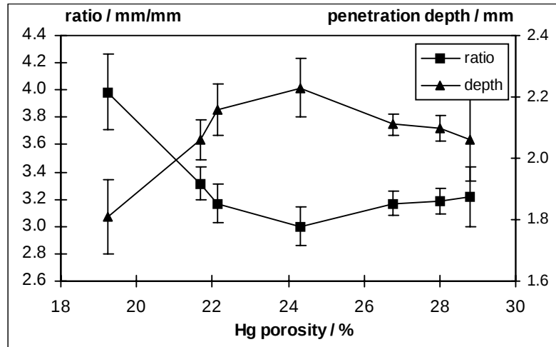
Fig. 15. Ratio of surface diameter to maximum penetration depth of a droplet shown as a function of the mercury porosity as measured from the identical series of compressed tablets
