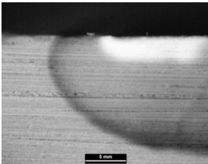
Fig. 9. Cross-section view (under fluorescence microscope) of the dyed tablet space of a blend of equal amounts of Rhodamin B (retarded) and Aluminumphthalocyanine-sodiumsulfonate (advanced) shows dramatically the chromatography effect (magnification 50x)
