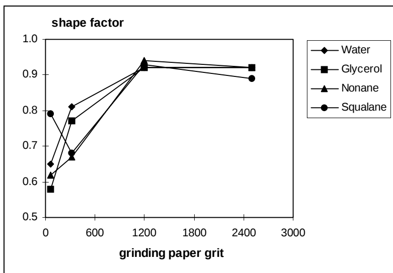
Fig. 10. With grit 1200, polished surfaces show maximum shape factor, which means maximum roundness/uniformity of the droplet stain
