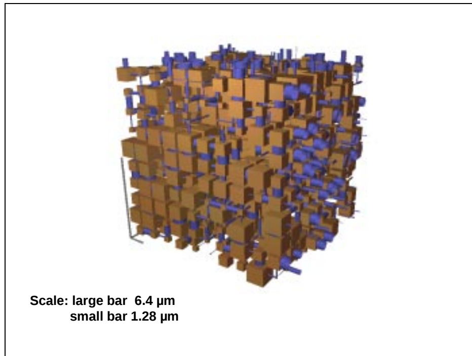
Fig. 19. Unit cell of a tablet consolidated at 57.6 MPa having a porosity of 28.7%
