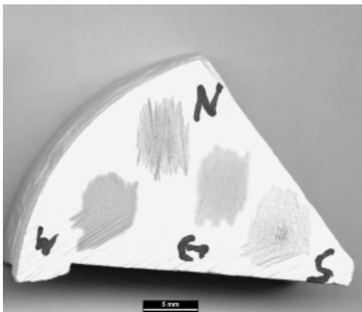
Fig. 11. Different stained liquids show strong influence of surface scratches (ground with 60-grit paper).
