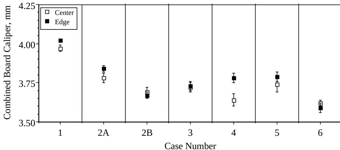
Figure 9. Caliper of Corrugated Board (as Measured in the Center and on the Edges of the Board) Plotted versus Corrugation Case Number.
