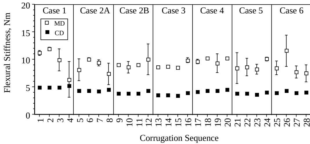
Figure 5. Flexural Stiffness of Corrugated Board (as Measured in MD and CD Directions) Plotted versus Corrugation Sequence.
