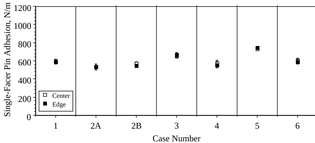
Figure 10. Single-Facer Pin Adhesion of Corrugated Board (as Measured in the Center and on the Edges of the Board) Plotted versus Corrugation Case Number.
