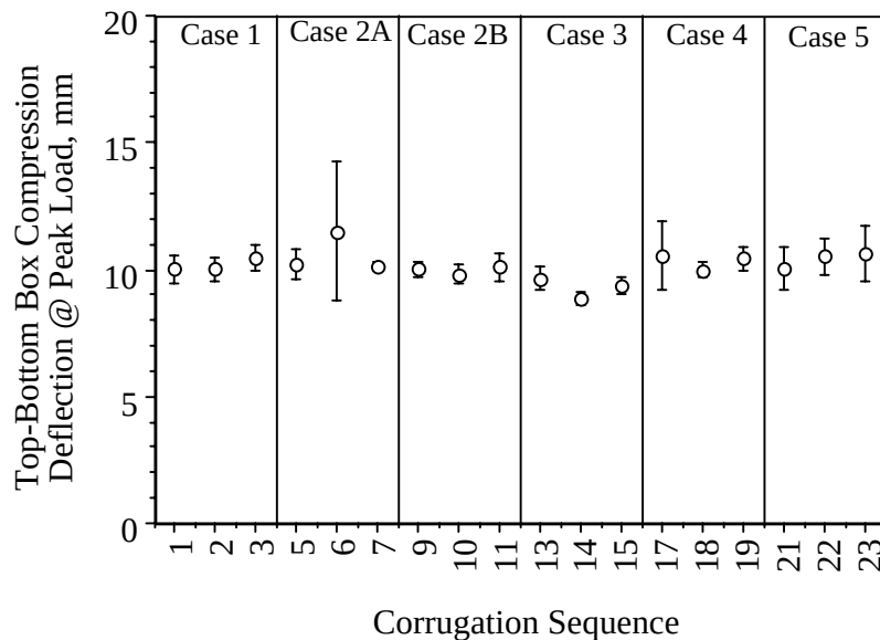
Figure 7. Top-To-Bottom Box Compression Deflection at Peak Load Plotted versus Corrugation Sequence.
