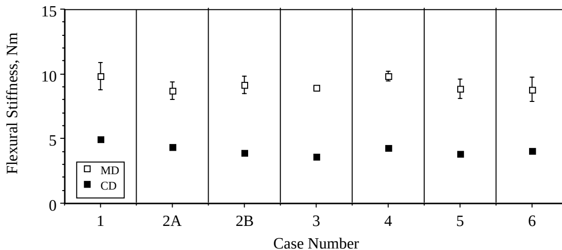
Figure 12. Flexural Stiffness of Corrugated Board (as Measured in MD and CD Directions) Plotted versus Corrugation Case Number.
