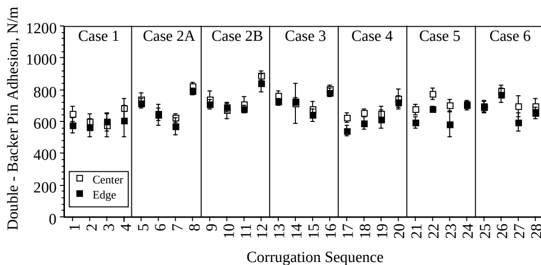
Figure 4. Double-Back Pin Adhesion of Corrugated Board (as Measured in the Center and on the Edges of the Board) Plotted versus Corrugation Sequence.
