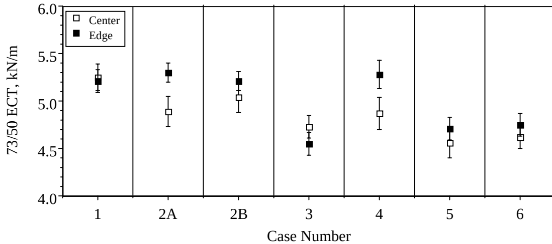
Figure 8. Edge Crush Test of Corrugated Board (as Measured in the Center and on the Edges of the Board) Plotted versus Corrugation Case Number.
