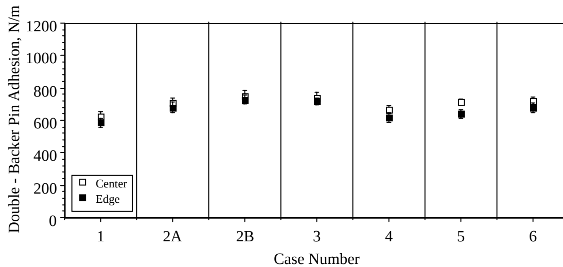
Figure 11. Double-Back Pin Adhesion of Corrugated Board (as Measured in the Center and on the Edges of the Board) Plotted versus Corrugation Case Number.
