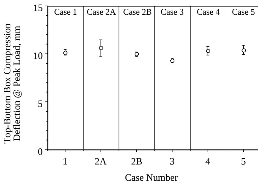
Figure 14. Top-To-Bottom Box Compression Deflection at Peak Load Plotted versus Corrugation Case Number.
