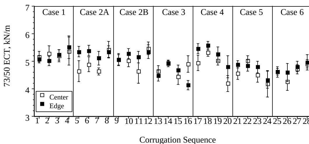
Figure 1. Edge Crush Test of Corrugated Board (as Measured in the Center and on the Edges of the Board) Plotted Versus Corrugation Sequence.
