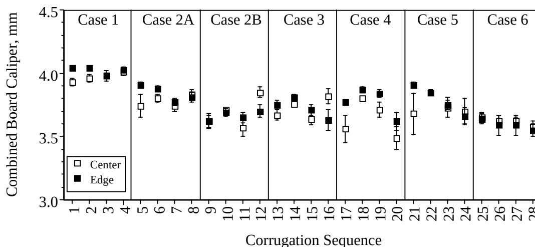
Figure 2. Caliper Of Corrugated Board (as Measured in the Center and on the Edges of the Board) Plotted Versus Corrugation Sequence.
