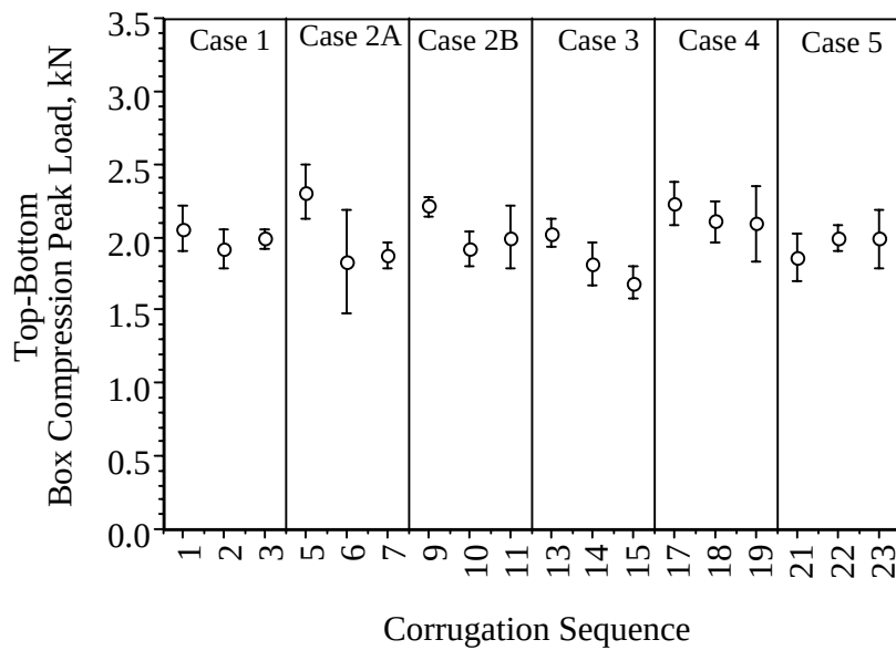
Figure 6. Top-To-Bottom Box Compression Peak Load Plotted versus Corrugation Sequence.
