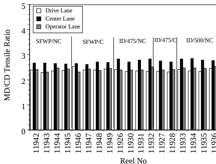
Figure 9. MD/CD Tensile Ratio Versus Reel Number.
