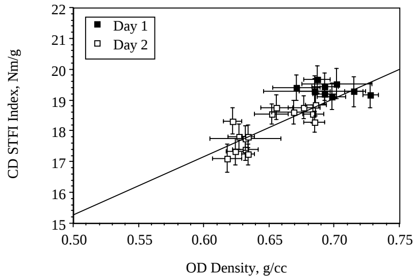
Figure 13. Cross-Directional STFI Compression Index versus OD Density.
