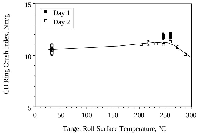
Figure 12. Cross-Directional Ring Crush Index versus Target Roll Surface Temperature.
