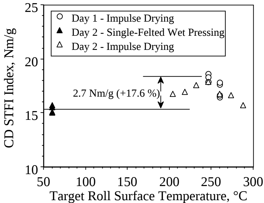
Figure 5. Preliminary Cross-Directional STFI Compression Strength Index versus Target Roll Surface Temperature.
