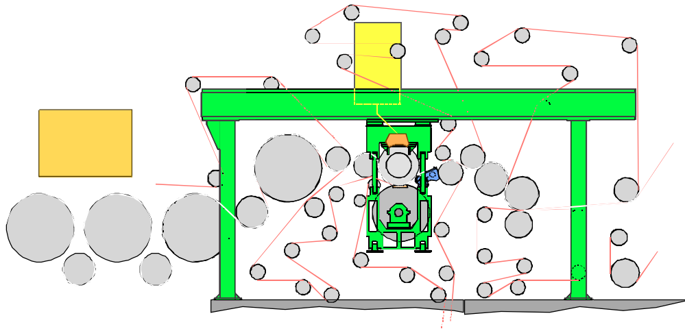
Figure 1. Press Section of the Pilot Paper Machine Showing the Impulse Dryer.
