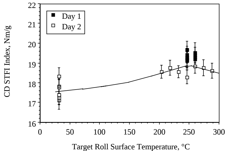
Figure 11. Cross-Directional STFI Compression Index versus Target Roll Surface Temperature.
