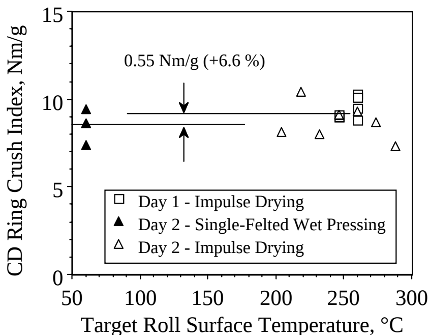
Figure 6. Preliminary Cross-Directional Ring Crush Index versus Target Roll Surface Temperature.
