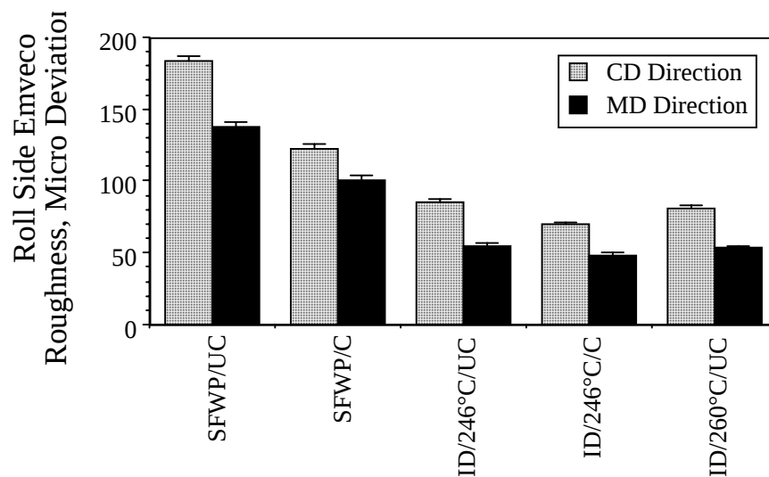
Figure 14. Micro Average Roll Side Emveco Roughness for Linerboard Production Cases.
