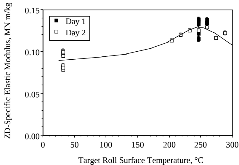
Figure 10. ZD- Specific Elastic Modulus versus Target Roll Surface Temperature.
