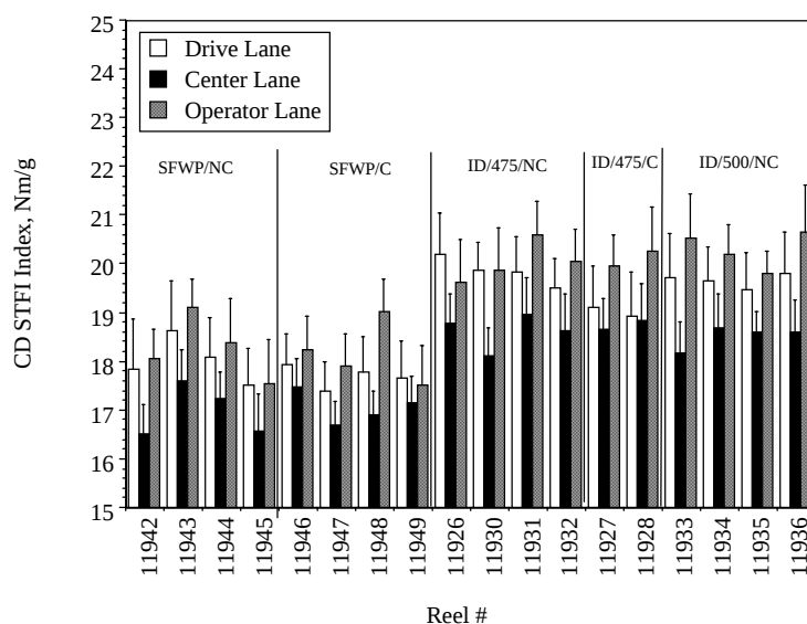
Figure 7. Cross-Directional STFI Index versus Reel Number.
