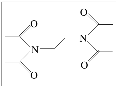
Scheme 9: Tetra acetyl ethylene diamine (TAED) (Croud and Mathews 1996).
