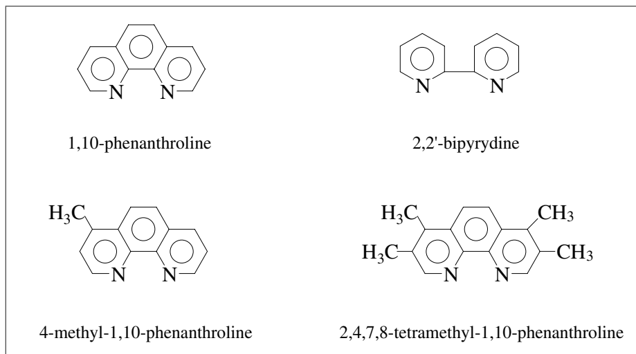
Scheme 11: Polypyridines containing an a,a' -diimine group as part of an aromatic system applied in various bleaching trials. (Jaschinski and Patt 1998).
