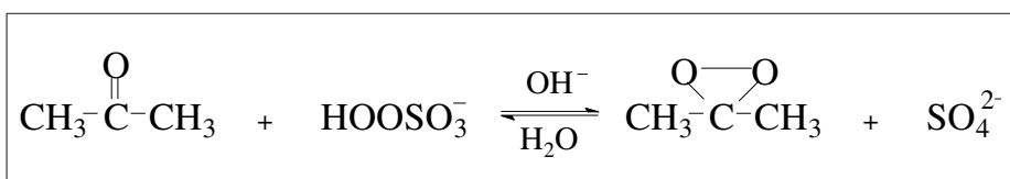
Scheme 13: Synthesis of dimethyldioxirane (DMD) from acetone and peroxymonosulfuric acid. (Lee et al. 1994)
