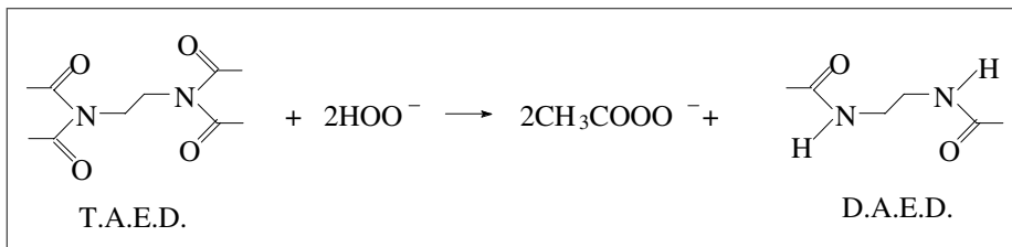
Scheme 10: The reaction of TAED with hydrogen peroxide under alkaline conditions. (Croud and Mathews 1996).
