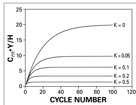
4. Effect of adsorption on the speed of substance buildup.
