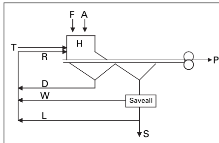
1. Water flows in a paper mill.
