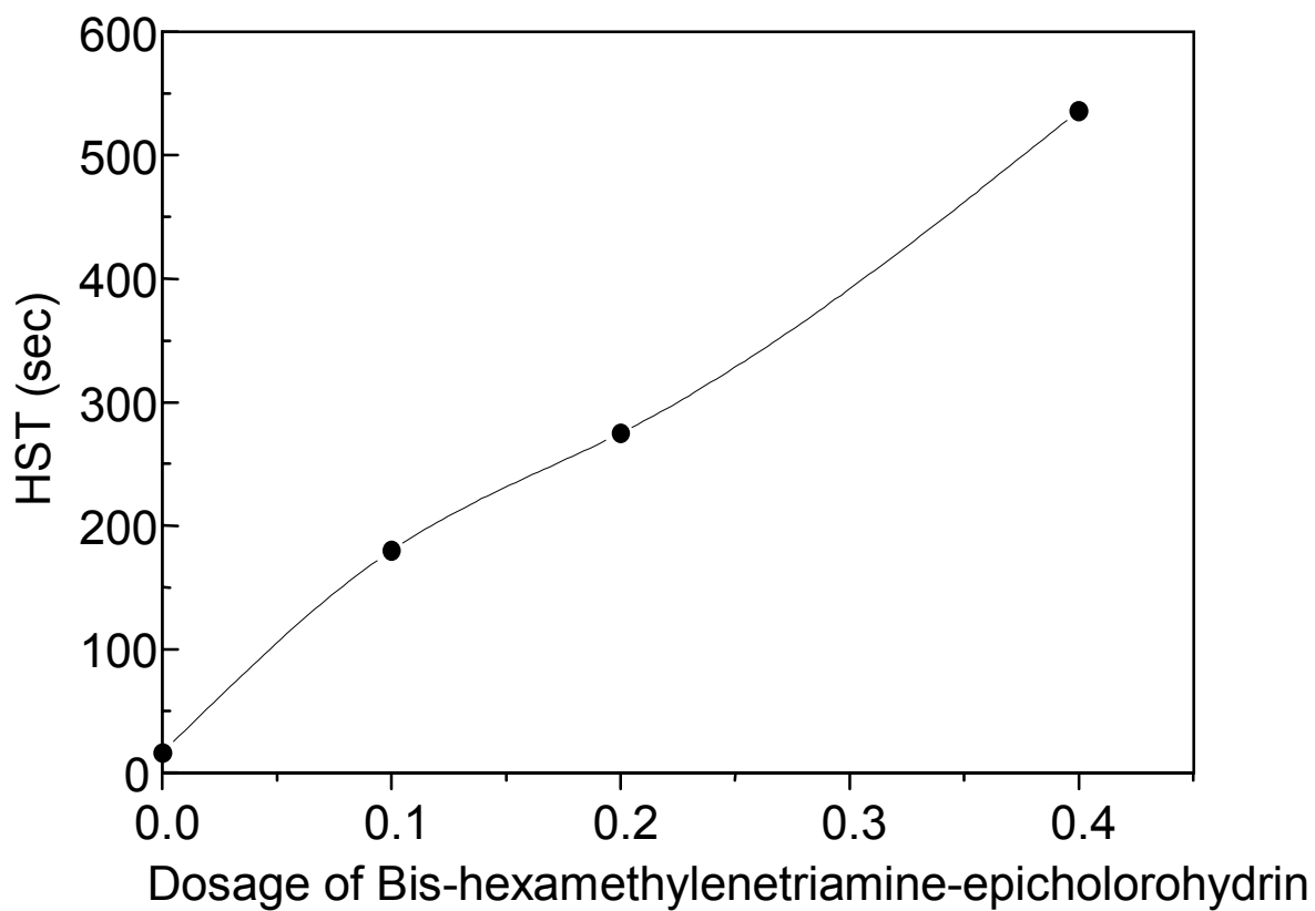
Figure 13 Effect of dosage of bis-hexamethylenetriamine-epichlorohydrin on rosin sizing at rosin (0.4%), alum (0.25%) and pH 7.5.
