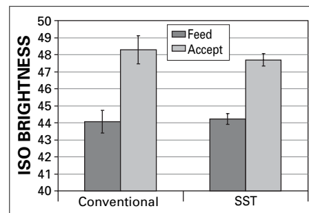
7. Brightness values obtained from pads prepared from the GSC feed and accept streams during conventional flotation deinking and during the incorporation of surfactant spray technology.
