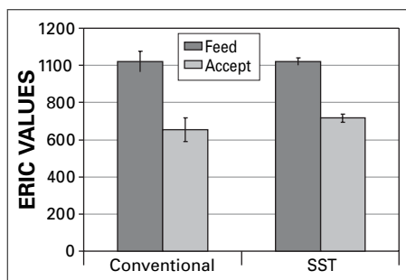
8. ERIC values obtained from pads prepared from the GSC feed and accept streams during conventional flotation deinking and during the incorporation of surfactant spray technology.
