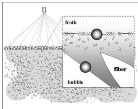
1. By applying frothing agent as a spray to the top of a conventional flotation cell, unfavorable interactions within the bulk pulp suspension may be avoided.
