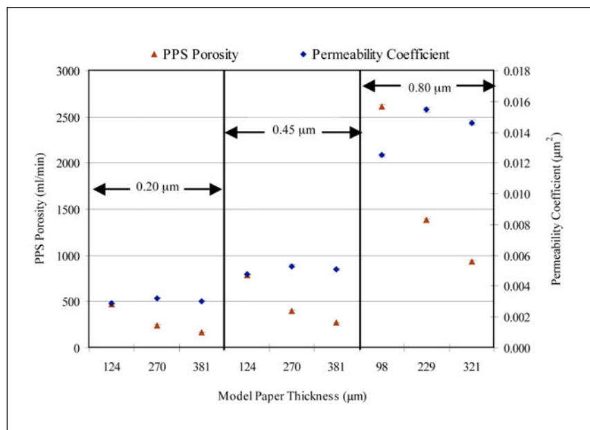
Figure 1. Comparison of permeability coefficients and PPS porosities of model papers
