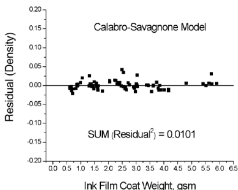
2. Sum of squares of reflection density residuals and their distribution for various models.
