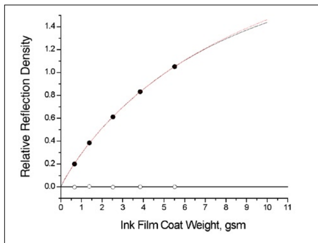
1. Ink mileage curve from sample 2 (the solid line is the curve fitted using the Oittinen model and the dotted line that fitted using the Calabro-Savagnone model).
