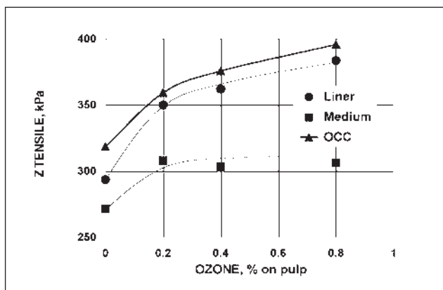
6. Z direction tensile strength vs. ozone charge.
