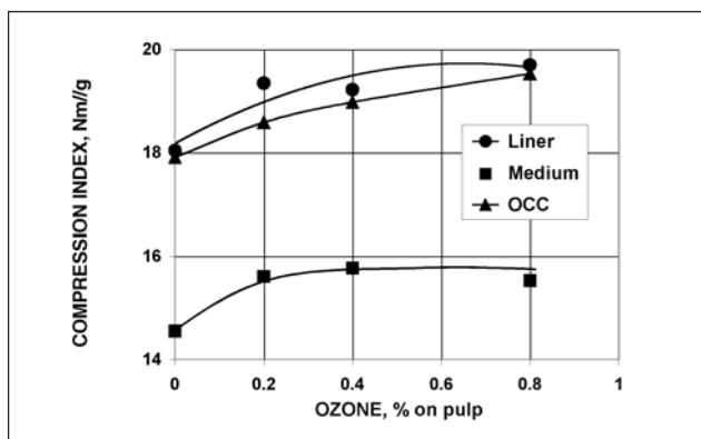
7. Short span compressive strength (SSCT) vs. ozone charge
