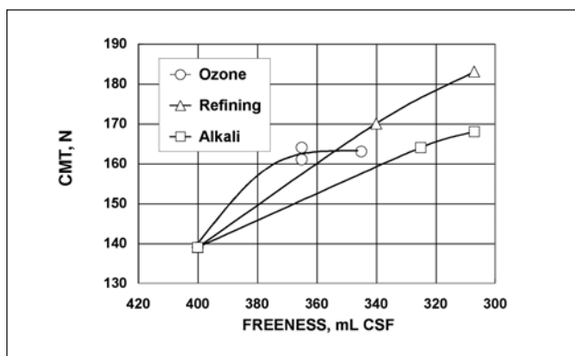
10. Concora crush value against freeness for the three treatments of the OCC pulp.
