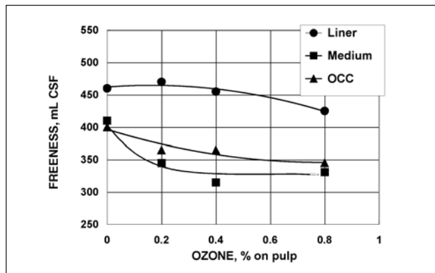
9. Freeness vs. ozone charge.
