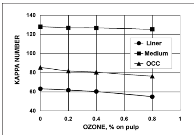
1. Kappa number as a function of ozone charge for pulps recycled from kraft liner, semichemical corrugating medium papers, and OCC.
