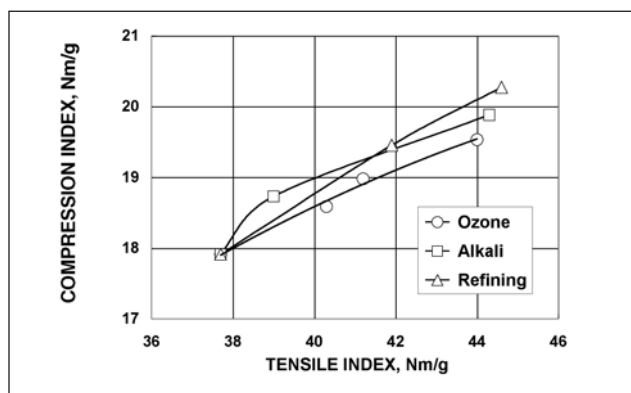
11. Comparison between the effects of ozone treatment (0.2, 0.4, and 0.8 % on pulp), alkali treatment (1.0 and 2.0 % NaOH on pulp) and refining on compressive and tensile strength of OCC pulp.
