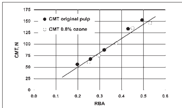
4. CMT value (130 g/m 2 handsheets) as a function of relative bonded area of the R30 fraction of the recycled pulp from liner paper.
