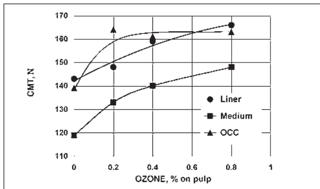
8. Concora crush resistance vs. ozone charge.
