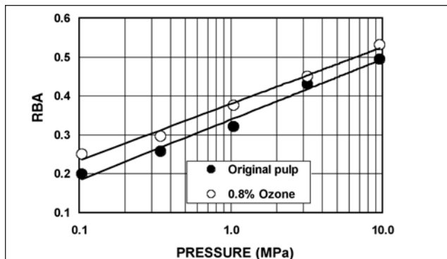
3. Relative bonded area estimated by Page model as a function of the pressing pressure.
