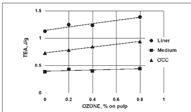
5. Tensile energy absorption vs. ozone charge (% on dry pulp).
