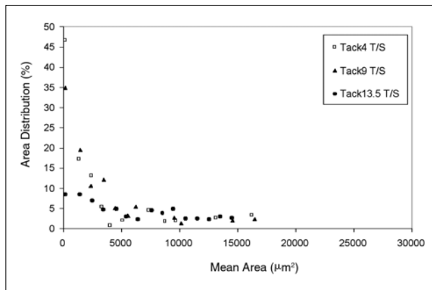
12. Man-Roland Uniset lint area distribution as a function of ink tack at 50% printing tone at a 27° take-off angle.
