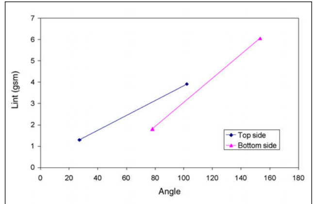
6. Effect of paper side and take-off angle on linting
