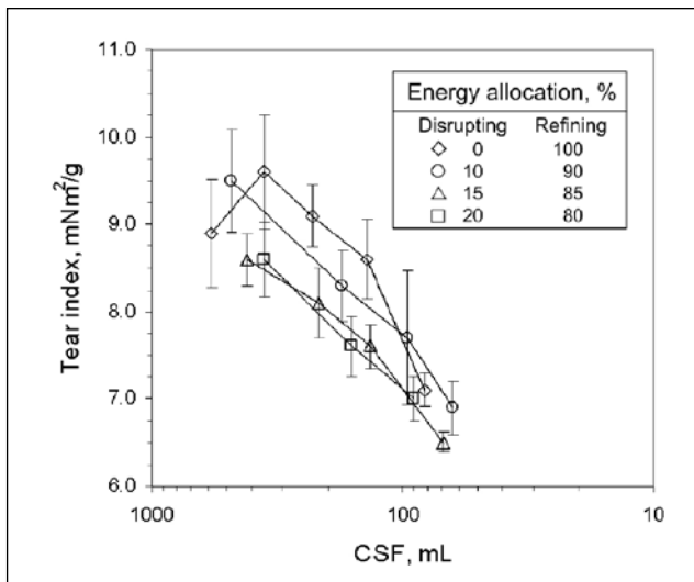
10. Tear resistance as a function of pulp freeness in second-stage refining.
