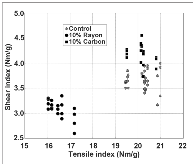
5. Tensile strength index vs. double-notch-shear (DNS) index for handsheds.
