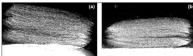
7. X-ray radiographs of eucalyptus handsheds containing 10% carbon fiber (a) or rayon fiber (b). The scale of the images is 1,400 \mu m horizontal by 840 \mu m vertical.
