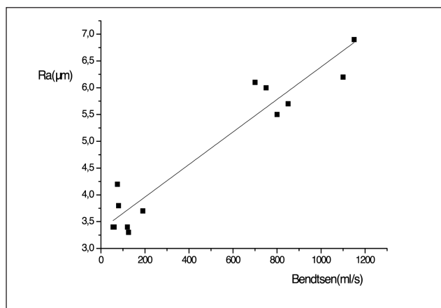
8. Ra using the confocal microscope versus the Bendtsen method ( r^2 = 0.91 ).
