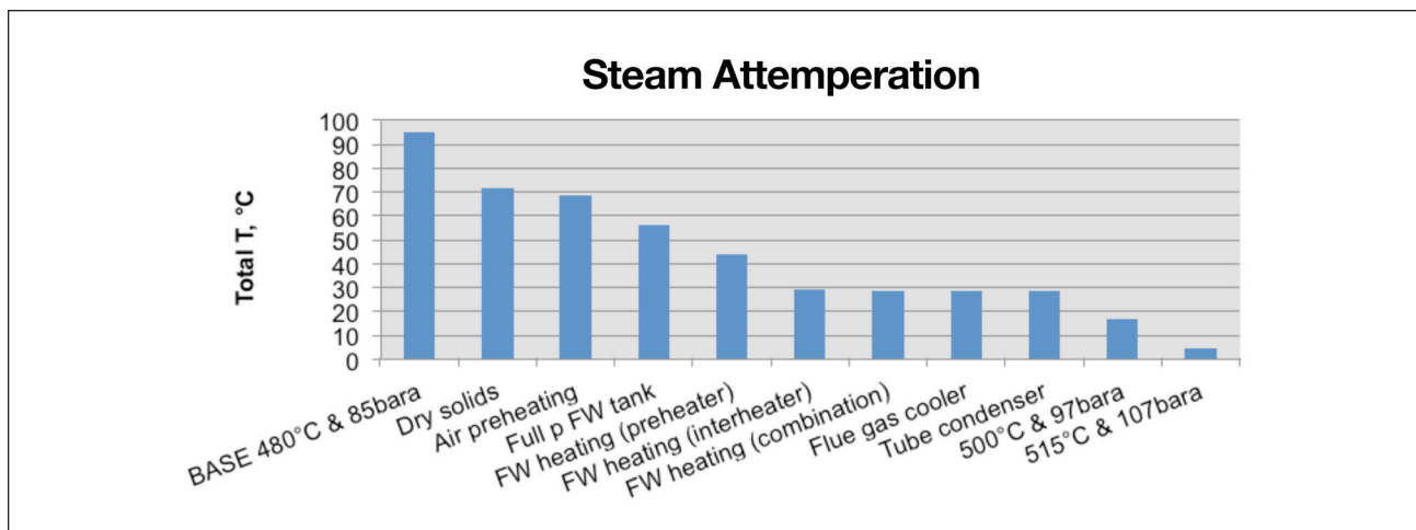
3. Cumulative effect of high power features on total boiler steam attenuation (FW = feedwater).
