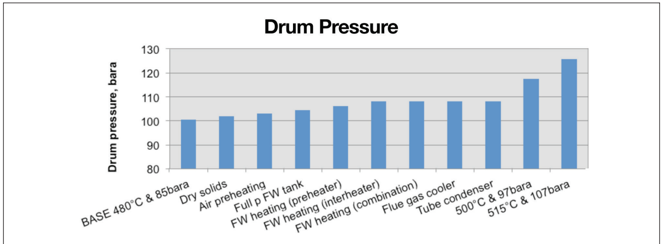
6. Cumulative effect of high power features on drum pressure (FW = feedwater).
