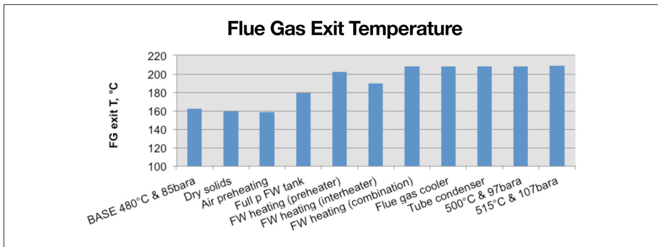
5. Cumulative effect of high power features on flue gas exit temperature (FW = feedwater).
