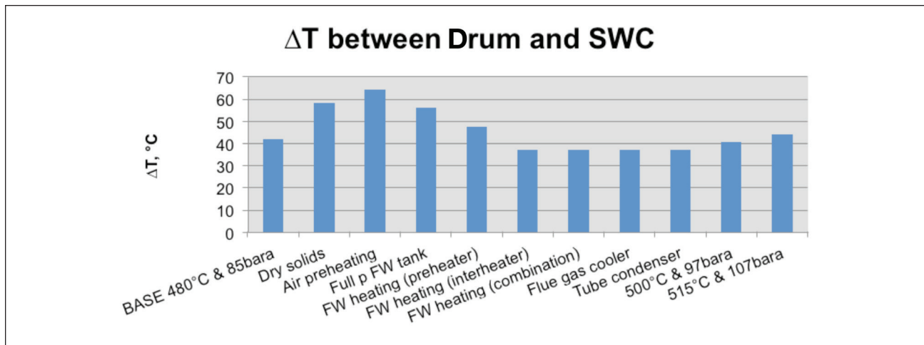
4. Cumulative effect of high power features on temperature difference between drum and SWC (SWC = sweet water condenser; FW = feedwater).
