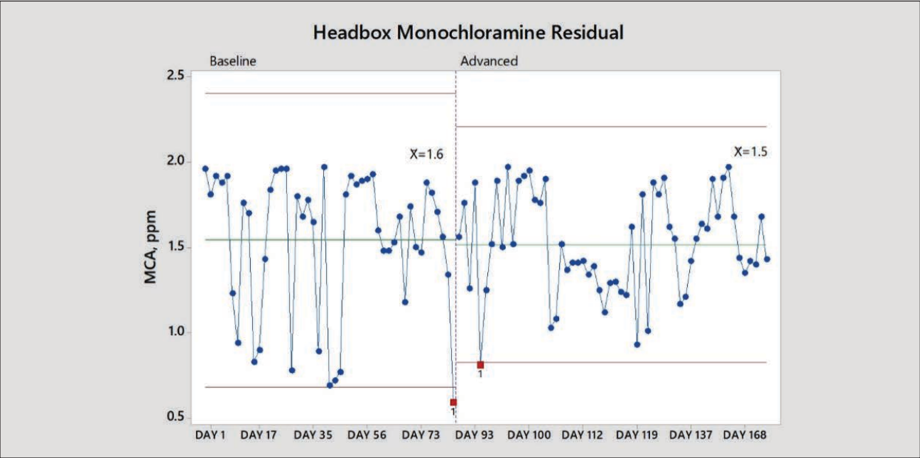
8. Phase 3 evaluation of headbox MCA residual. Although the headbox residuals were similar for both the baseline and advanced control dosing modes, the standard deviation for the baseline was 0.4 ppm compared to 0.3 ppm for the advanced control period.
