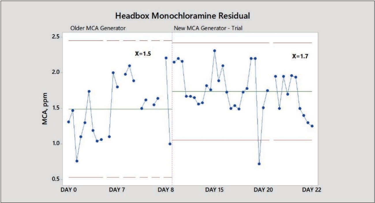
2. Phase 1 trial evaluation of headbox MCA residual. When comparing the performance of the new generator with the older generator, similar MCA residuals were achieved during both periods.
