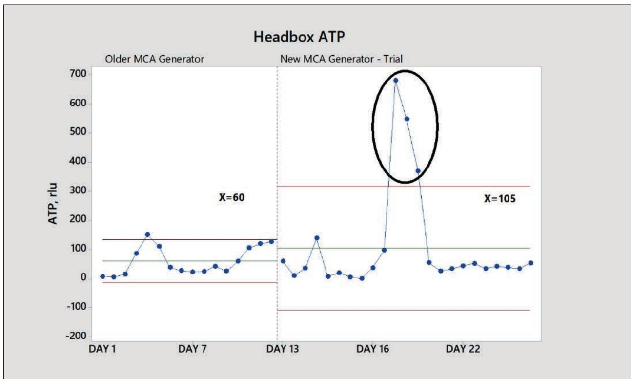
4. Phase 1 trial evaluation of microbial control via adenosine triphosphate (ATP) analysis. With the older generator, ATP numbers measured at the headbox were well below the mill's established upper limit of 500 relative light units (rlu). The new generator produced similar results. The three outliers (circled) occurred after an unplanned downtime and correlate to slightly lower MCA headbox residuals during the same time period (Fig. 1).
