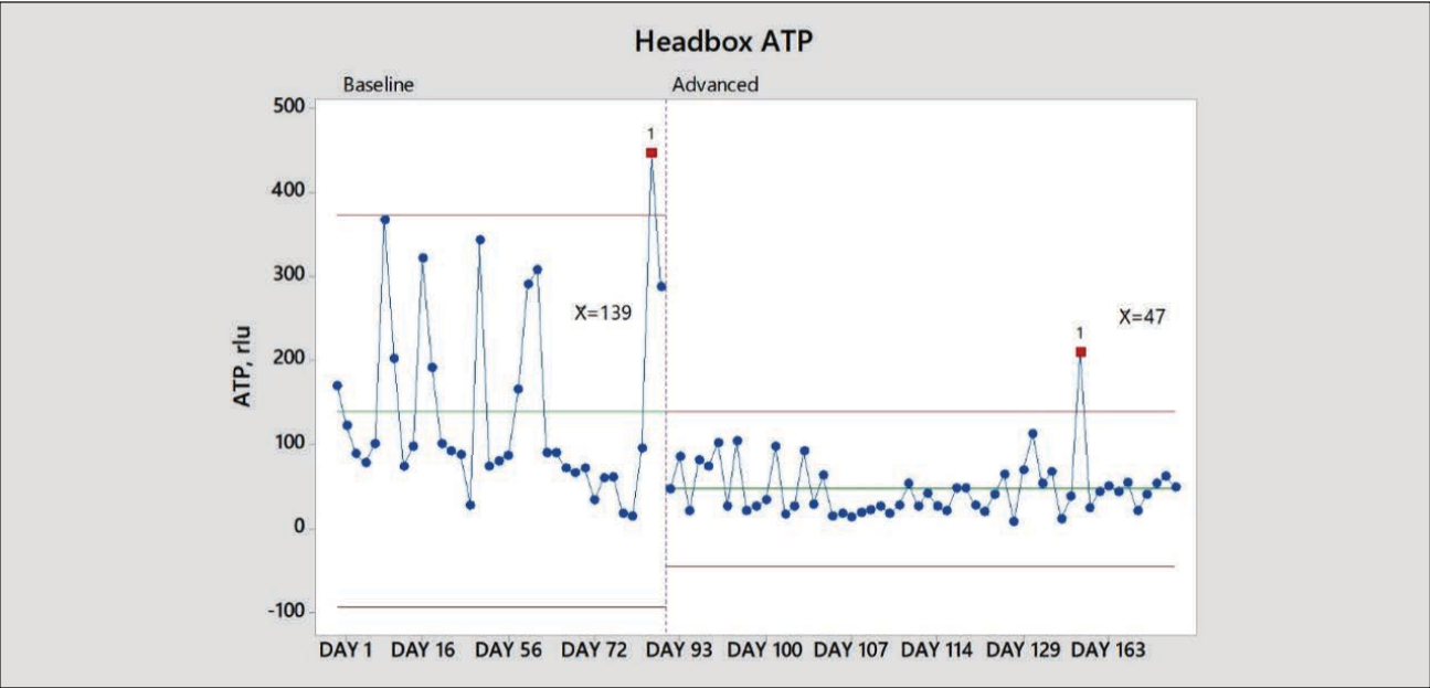
9. Phase 3 evaluation of headbox ATP. Both dosing modes resulted in headbox ATPs below the mill's requirement. Lower variability was achieved with the advanced control dosing mode.
