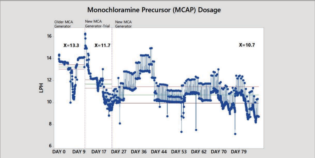
6. Phase 2 evaluation of MCAP dosage rate. The MCAP chemical dosage rate was reduced further while the MCA headbox residuals were maintained (Fig. 5).
