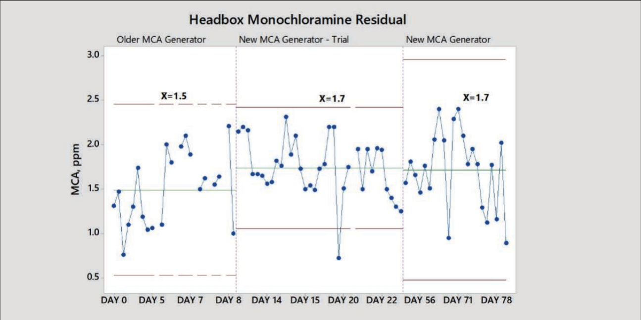
5. Phase 2 evaluation of headbox MCA residual. The headbox residuals were maintained during this phase while the MCAP flow rate was further reduced (Fig. 6).
