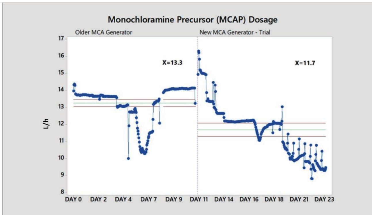
3. Phase 1 trial evaluation of monochloramine precursor (MCAP) dosage rate. For the new generator, the MCAP chemical flow rate was reduced while maintaining a similar headbox MCA residual (Fig. 2) as compared with the older generator.
