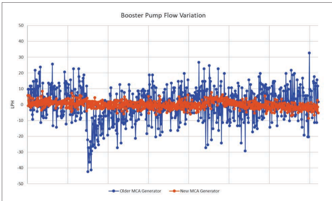
7. Phase 2 evaluation of the proportional–integral–derivative (PID) flow control valves. The water booster pump variation over a 12-h period was compared between the older and new generators. The flow variation was reduced by 75% due to the use of the PID flow control valves in the new unit.
