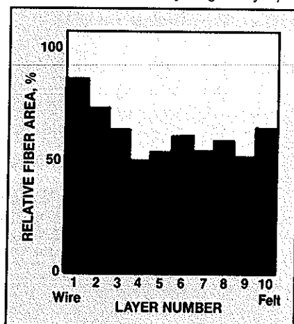
8. The relative density distribution in the z -direction of a LWC basesheet with MD microstriations (as determined by image analysis).
