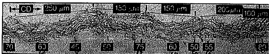
5. Cross section taken across the MD microstriations, where the lower numbers indicate sheet thickness in \mu\text{m}
