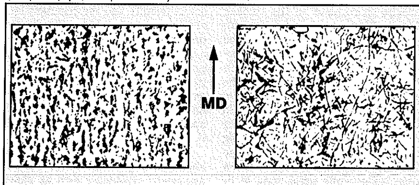
3. Enhanced images of paper (left) and used felt (right) in contact with glass plate under pressure (200 psi for paper, 1200 psi for the felt) show no correlation.
