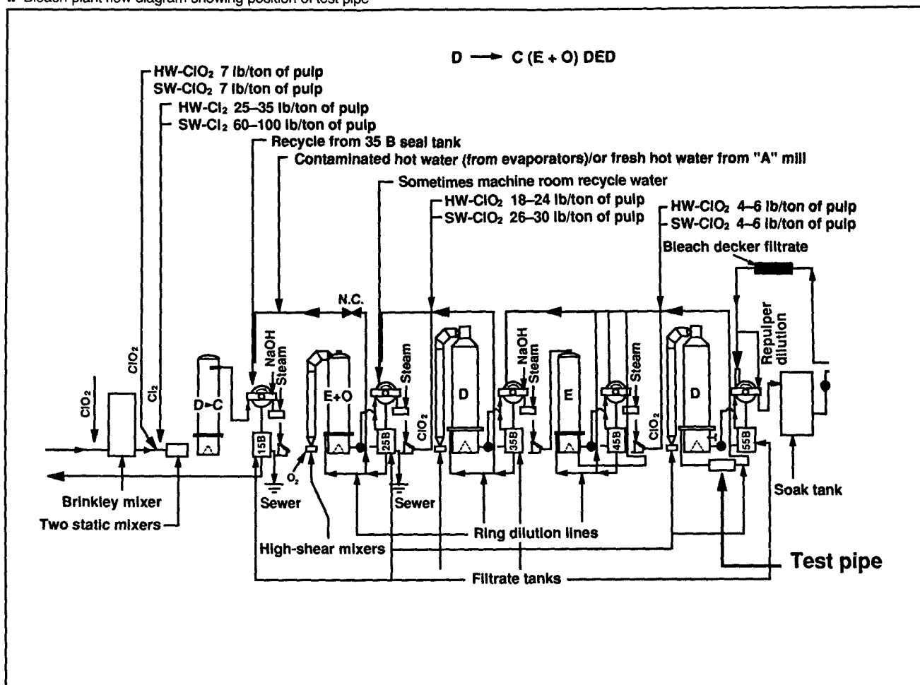
1. Bleach plant flow diagram showing position of test pipe
