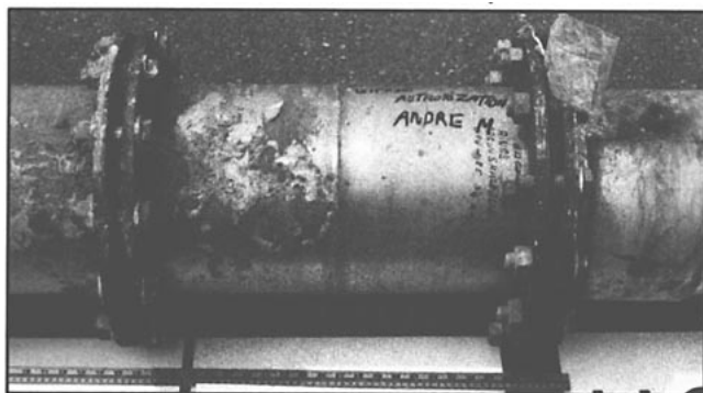
3. A cleaned circumferential weld of AL-6XN showing pitting. Pits initiated in unmixed zones of weld metal and spread under the corrosion products to nearby base metal.
