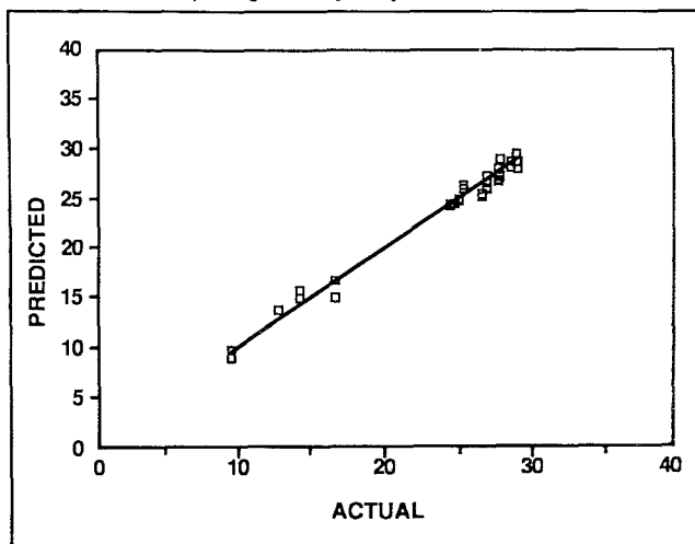
2. Confirmation of pine lignin analysis by NIR
