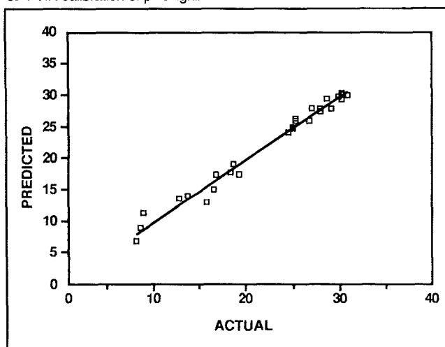
3. FTIR calibration of pine lignin
