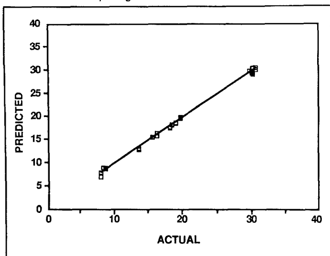
1. NIR calibration of pine lignin
