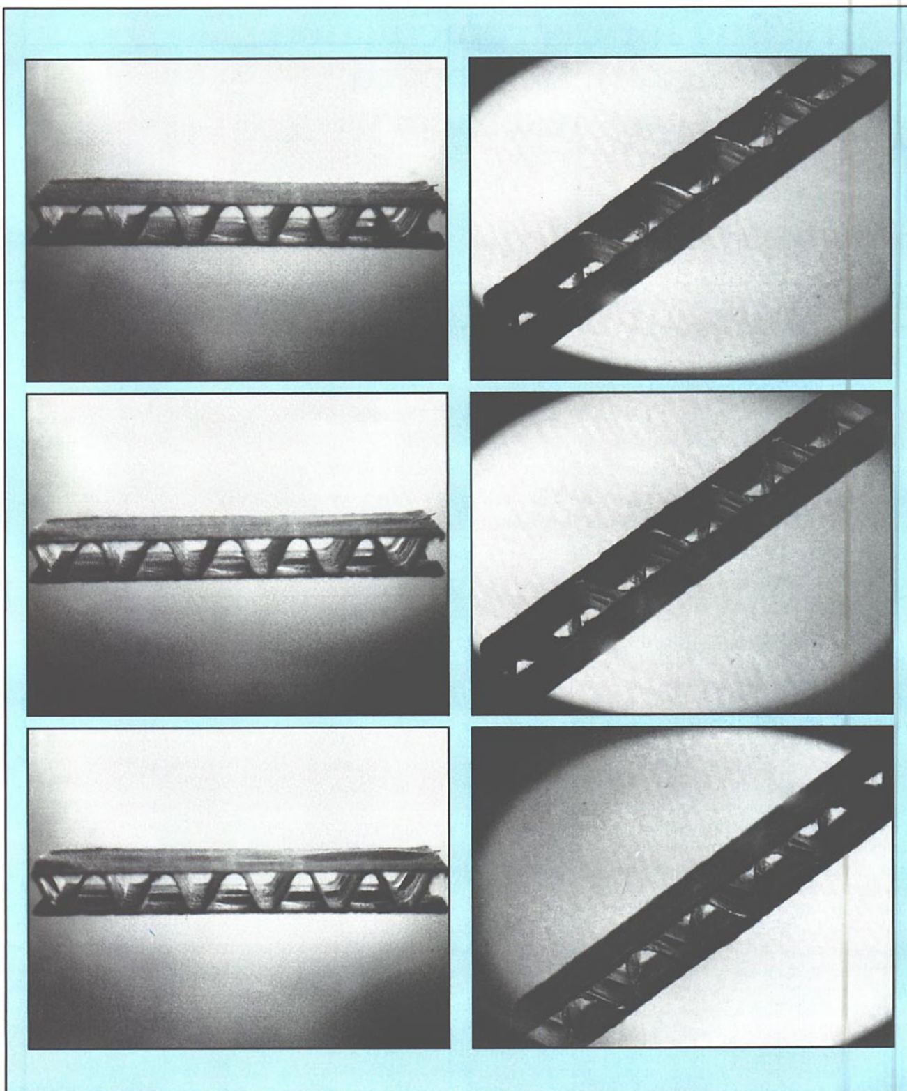
1. Progression of localized buckling in corrugated fiberboard short columns from a stable configuration to a postbuckled failure mode. In A, the facings buckle first; in B, the core buckles first. Compression is between two glass platens with a view through the flutes.
