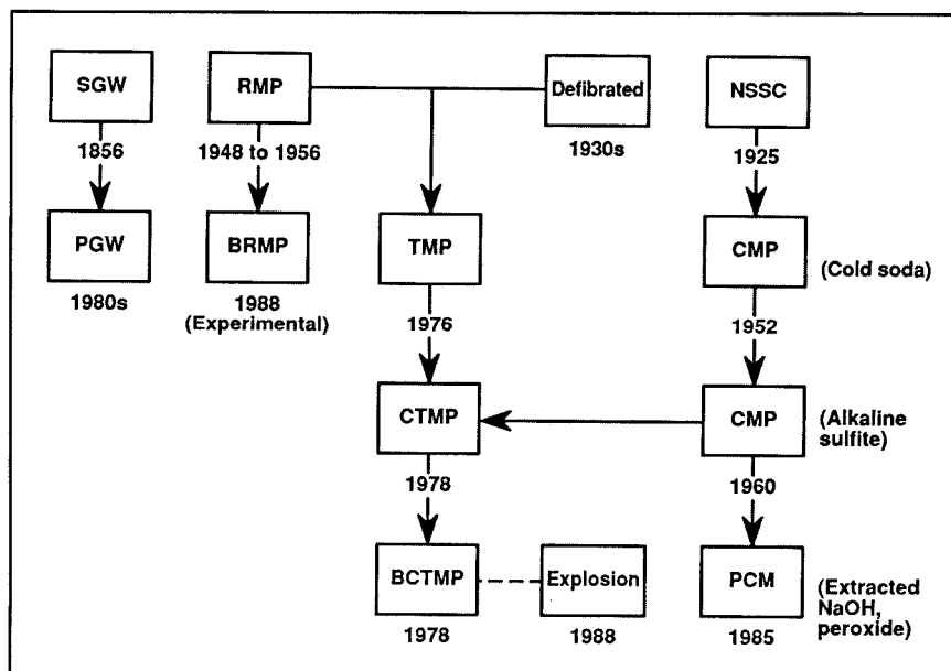
1. Development and interrelationships of ultra-high-yield pulping processes
