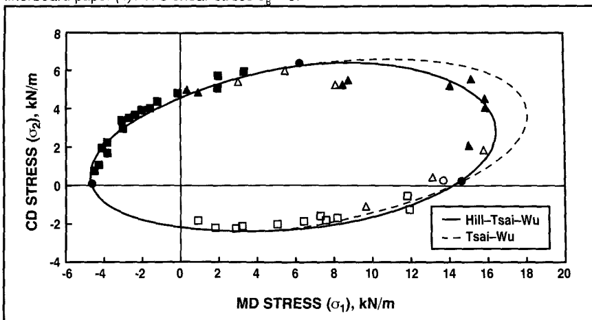
2. Plots of Hill-Tsai-Wu and Tsai-Wu failure criteria based on biaxial-strength data for linerboard paper (4). The shear stress \sigma_6 = 0 .
