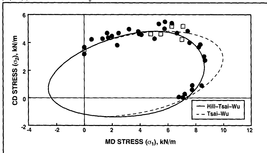
1. Plots of Hill-Tsai-Wu and Tsai-Wu failure criteria based on biaxial-strength data for sack paper (3). The shear stress \sigma_6 = 0 .
