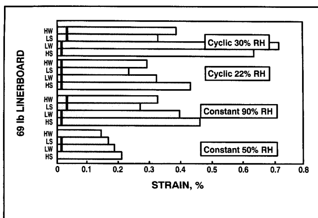
15. Median strain of 69-lb linerboard in CD
