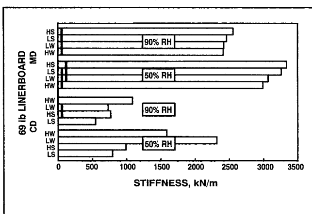
12. Mean stiffness of 69-lb linerboard
