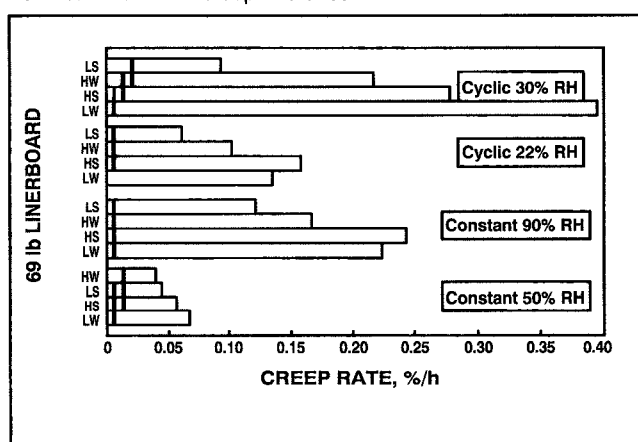
13. Mean maximum creep rate of 69-lb linerboard in CD
