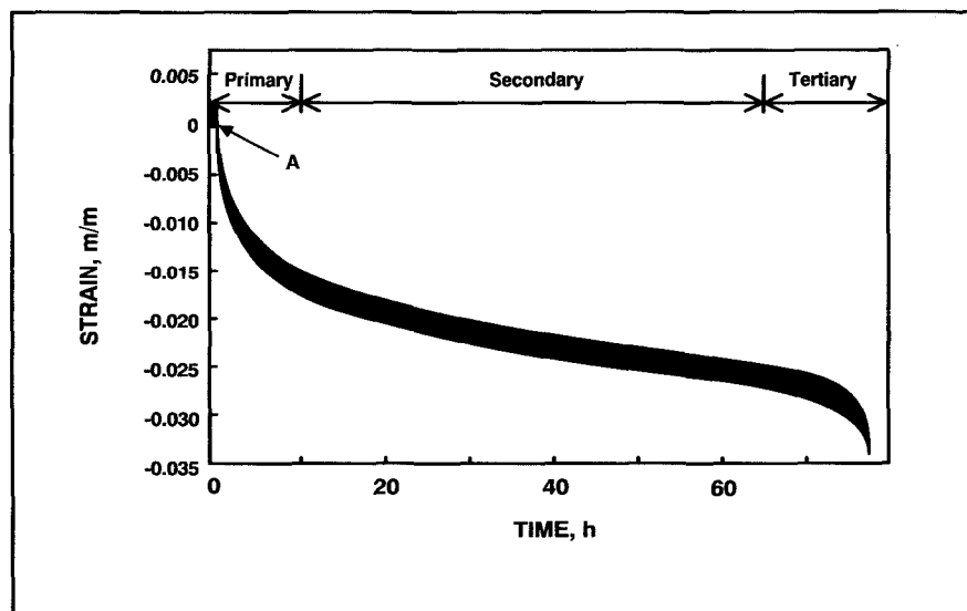
3. Typical compressive creep test
