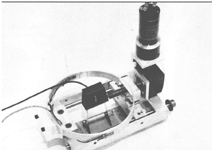
3. Typical compressive creep test
