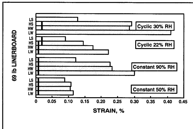
16. Median strain of 69-lb linerboard in MD
