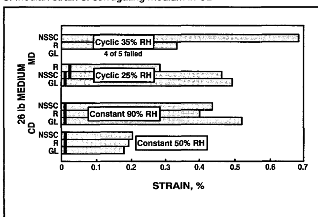
8. Median strain of corrugating medium in CD
