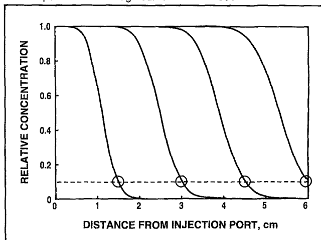
17. Computed breakthrough curves for P = 1000
