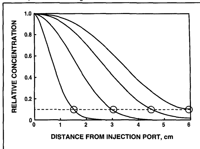
15. Computed breakthrough curves for P \approx 10
