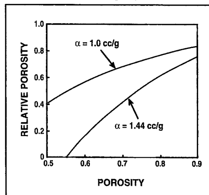
18. Predicted relative porosity results based on 90% of extrafiber pore space being open to flow. (Compare to Fig. 2.)
