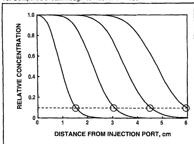
16. Computed breakthrough curves for P = 100
