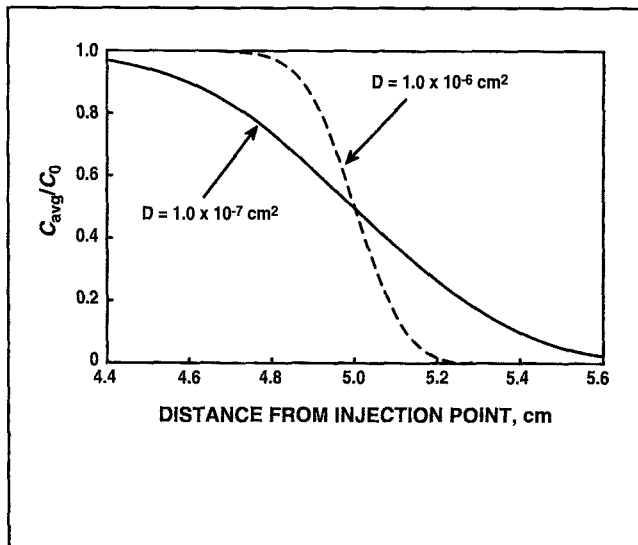
13. Predicted dispersion of a dye boundary after 5-cm travel in a capillary tube
