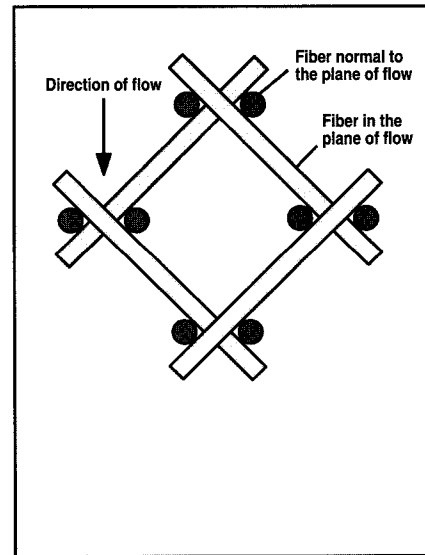
3. Unit cell of a fibrous medium used in the analysis of Kyan et al. (10)
