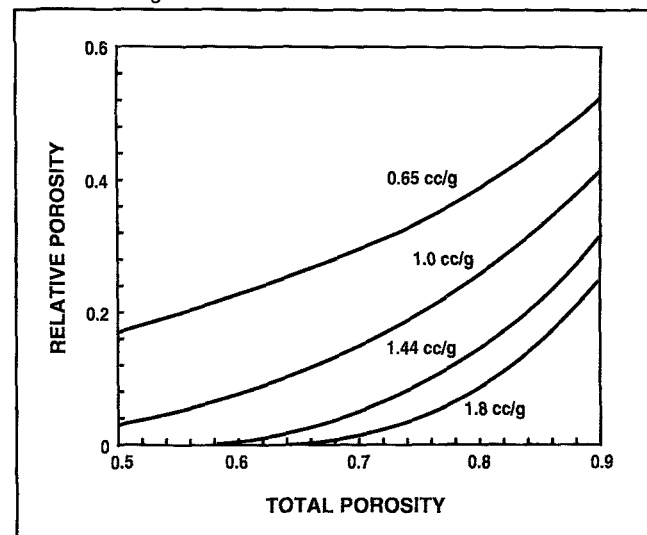
5. Relative porosity results based on a combination of Kyan's model (10) and extrafiber porosity analysis. Unhydrated fiber corresponds to \alpha = 0.65 cc/g.
