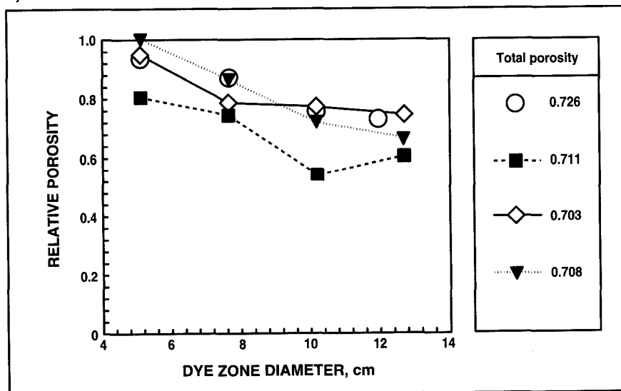
11. Relative porosity results in saturated blotter paper as a function of dye zone diameter injected into the sheet
