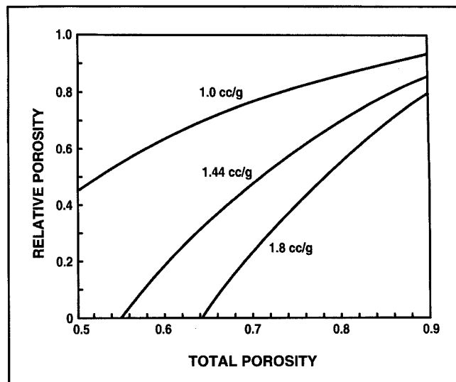
2. Relative porosity in paper based on Kozeny-Carman analysis using typical specific volume results
