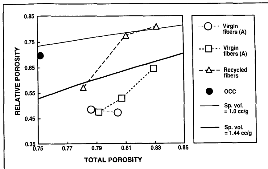
10. Relative porosity in virgin and recycled unbleached kraft sheets. Extrafiber pore space curves are also shown (see Fig. 2).
