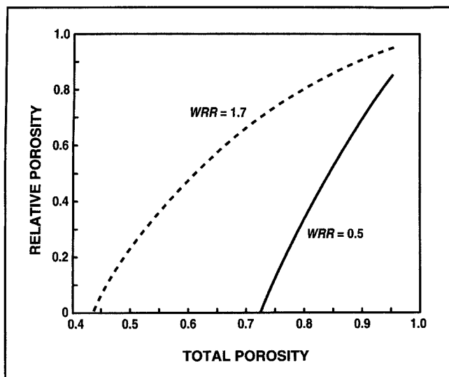
1. Estimated relative porosities from Eq. 2 for two WRR values
