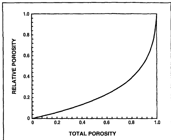
4. Predicted relative porosity based on the approach of Kyan et al. (10)
