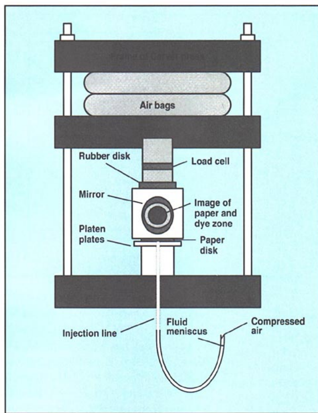
6. Modified lateral flow apparatus for dye injection tests
