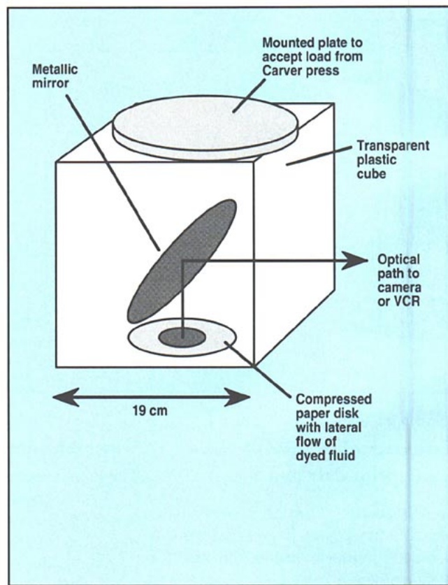
7. Plastic pressing block with mirror for optical access to a compressed sheet
