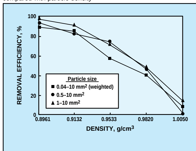
3. Effect of particle size on removal efficiency based on speck area compared with particle density
