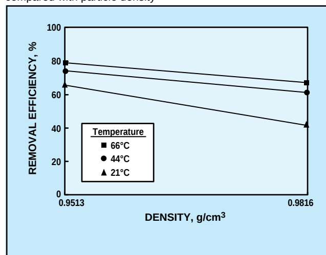
4. Effect of temperature on removal efficiency based on speck area compared with particle density
