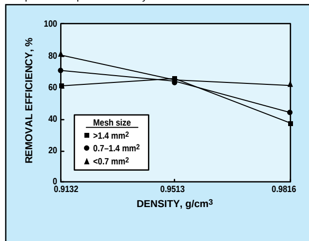
2. Effect of particle size on removal efficiency based on speck count compared with particle density
