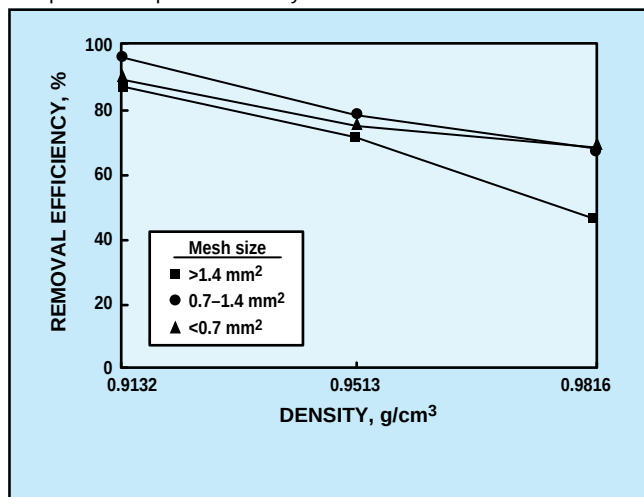
1. Effect of particle size on removal efficiency based on speck area compared with particle density
