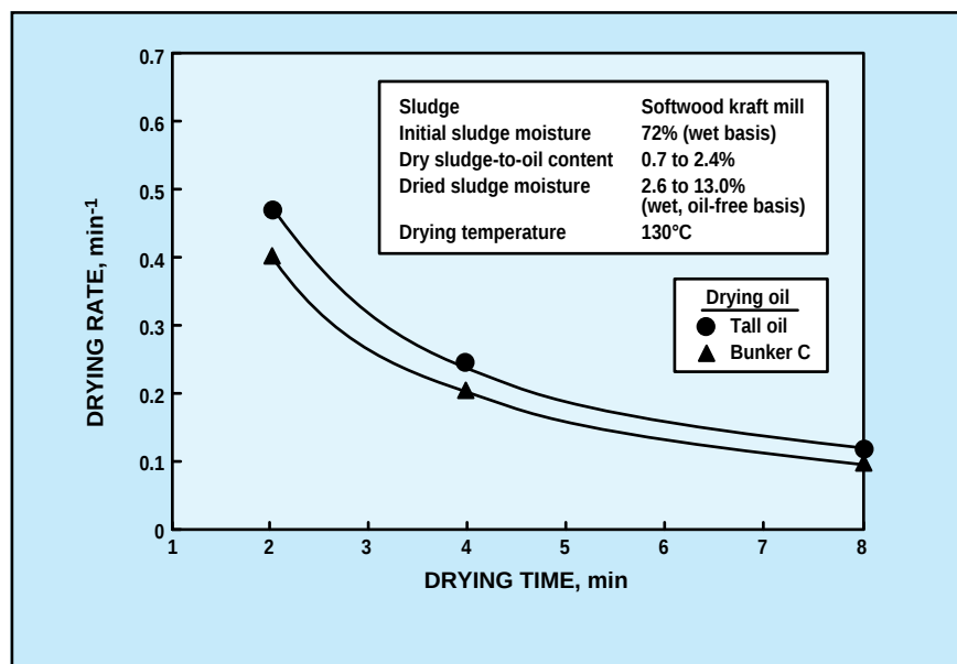
3. Overall drying rates of softwood kraft mill sludge as a function of drying time and type of oil used
