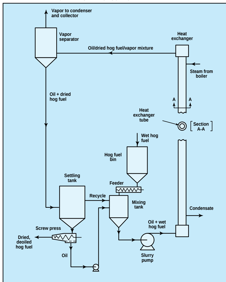
1. Schematic of the Paprican hog-fuel drying pilot plant
