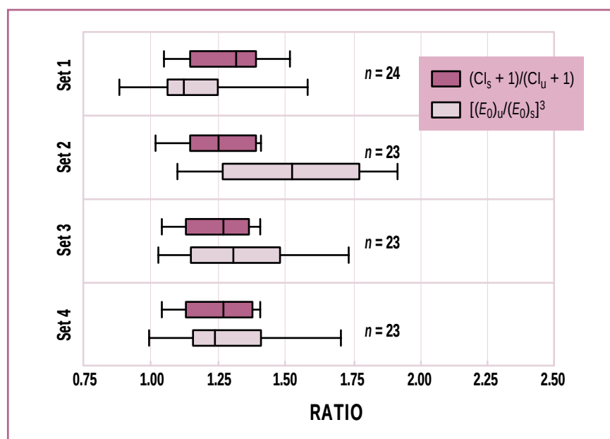
3. Comparison of (CI_s + 1)/(CI_u + 1) and [(E_0)_u/(E_0)_s]^3 for Sets 1–4. Data are presented in the form of box-and-whisker plots, with the box representing the interquartile range (25% to 75%) and the median displayed within.
