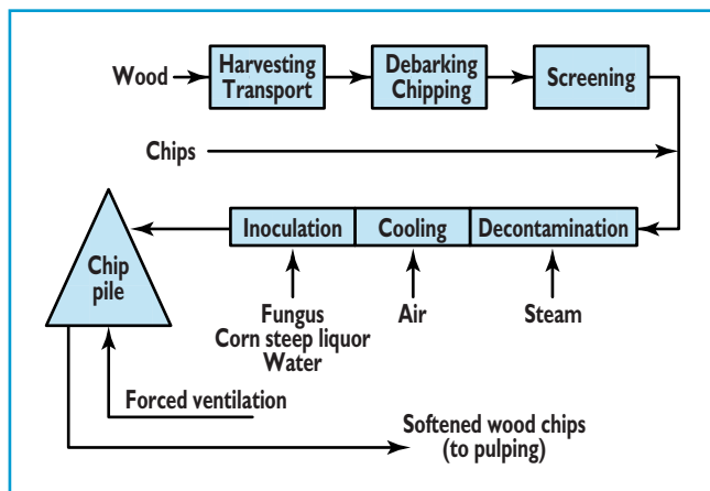
I. Overview of the biopulping process, showing how the biotreatment process fits into the wood-handling system of an existing mill
