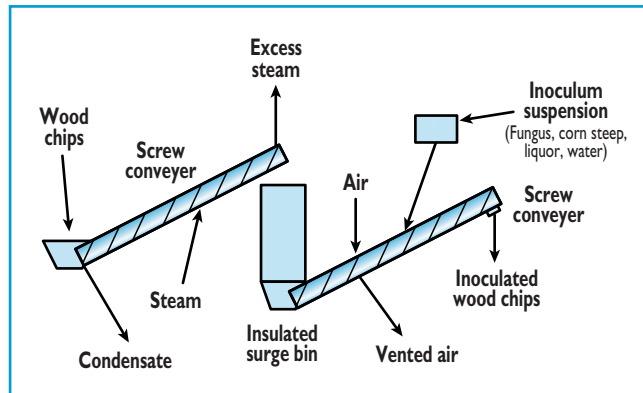
2. Continuous treatment system to decontaminate and inoculate wood chips. Wood chips are steamed in the first conveyor auger before being placed into a surge bin. The second screw conveyor then picks up the chips, cools them, and applies the inoculum.
