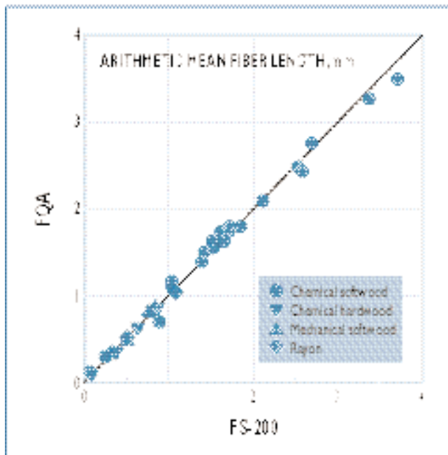
1. Arithmetic mean fiber length as measured by FQA and FS-200 for various pulp fractions and debris-free whole pulps (37 samples). Error bars in this and subsequent figures depict 95% confidence limits on the mean. Note that error bars may be smaller than the symbols
