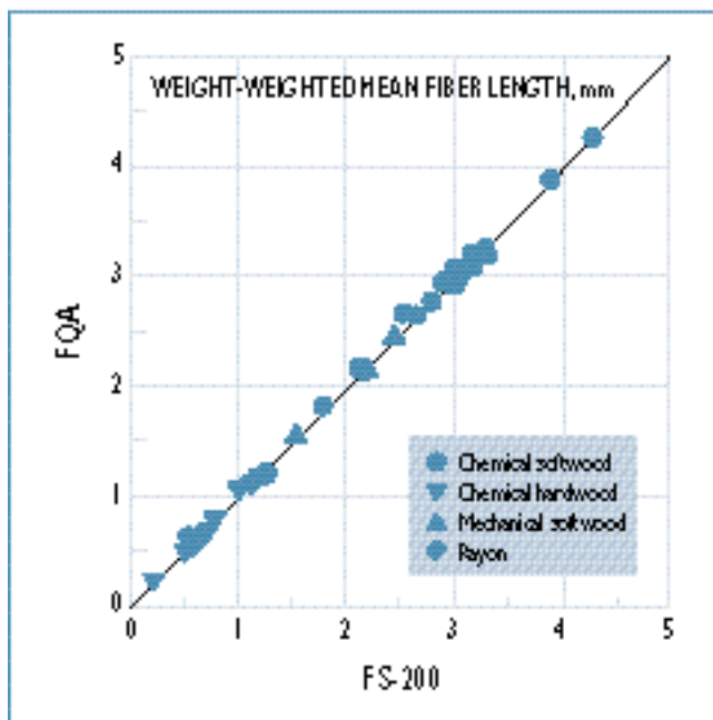
3. Weight-weighted mean fiber length as measured by FQA and FS-200 for various pulp fractions and debris-free whole pulps (37 samples)
