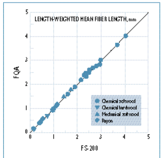
2. Length-weighted mean fiber length as measured by FQA and FS-200 for various pulp fractions and debris-free whole pulps (37 samples)
