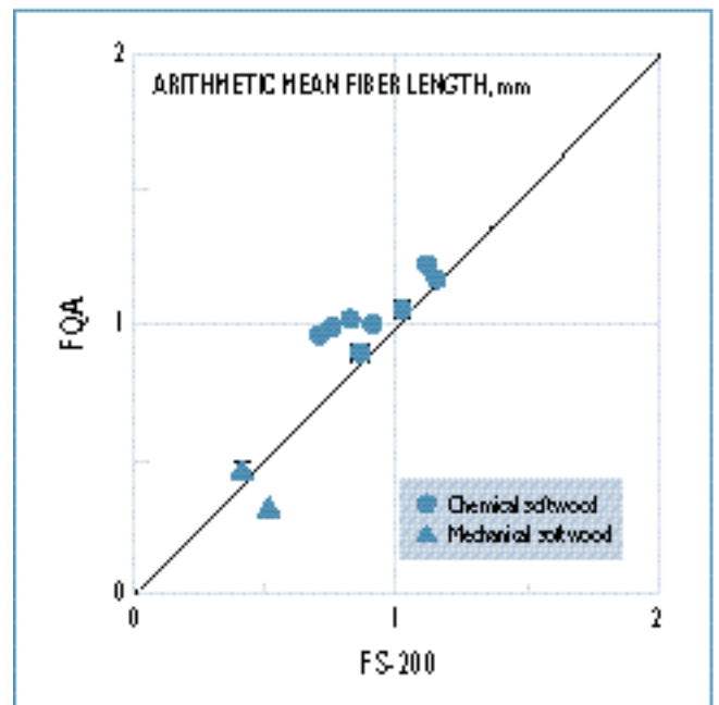
4. Arithmetic mean fiber length as measured by FQA and FS-200 for whole pulps (10 samples)
