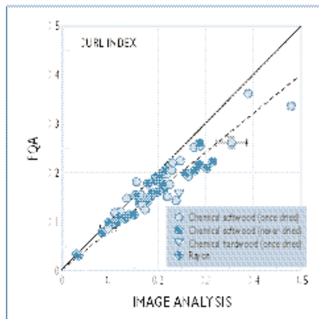
10. Curl index as measured by FQA and manually (image analysis) for various pulp fractions and debris-free whole pulps (54 samples)
