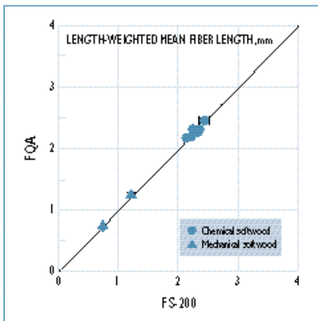
5. Length-weighted mean fiber length as measured by FQA and FS-200 for whole pulps (10 samples)
