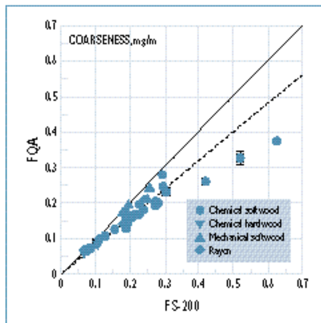
8. Coarseness as measured by FQA and FS-200 for various pulp fractions and debris-free whole pulps (36 samples)
