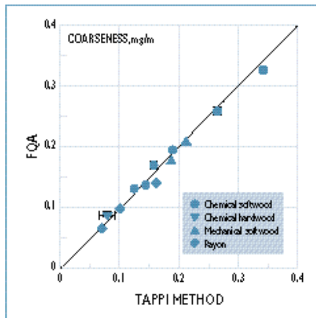
6. Coarseness as measured by FQA and TAPPI T 234 cm-84 for various pulp fractions and debris-free whole pulps (12 samples)
