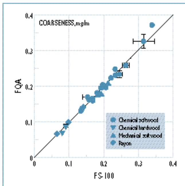
7. Coarseness as measured by FQA and FS-100 for various pulp fractions and debris-free whole pulps (27 samples)
